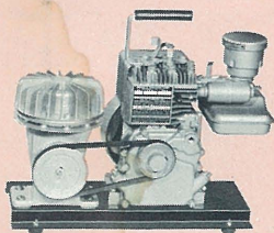
"HOOKAH" COMPRESSOR
