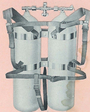
DOUBLE TANK BLOCK "SJ2" ASSEMBLY—
