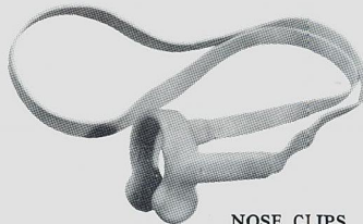
NOSE CLIPS
