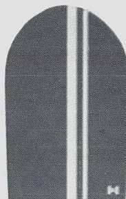
SKI DOOTER
