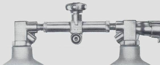
TWIN "J" VALVE
