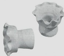
EAR STOPPLES
