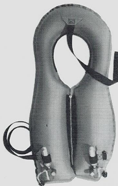
COMPETITION JACKETS
