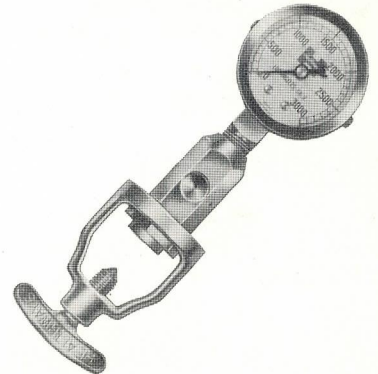
No. 1614 PRESSURE GAUGE AND YOKE WITH BLEEDER VALVE $9.95
