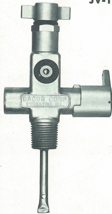
"LOW BOY" Spring loaded reserve valve. Bright chrome finish. Large round knurled shut-off knob. 300 P.S.I. reserve. New simplified design for accuracy and service free operation. JV-1 $29.50
