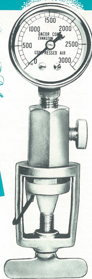
DELUXE PRESSURE GAUGE PG-C $11.95 All brass construction, satin chrome plated. Body machined from solid brass bar stock. Forged yoke and screw. Large knurled relief screw for easy turning. Yoke swivels, enabling gauge to be turned for reading.
